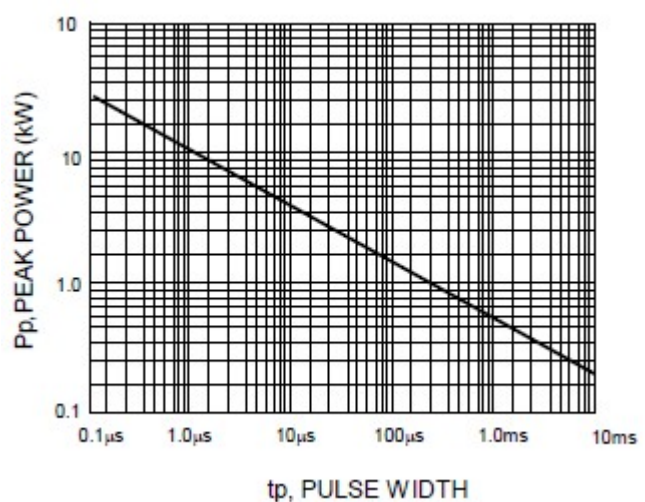
FIG.4 - PULSE RATING CURVE
