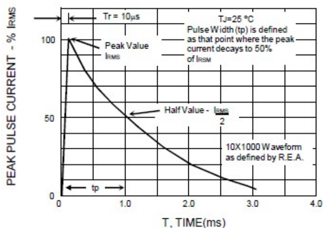
FIG.5 - PULSE WAVEFORM
