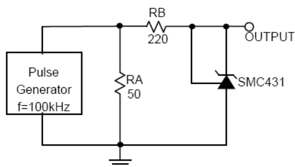
Fig. 13 Test Circuit For Pulse Response
