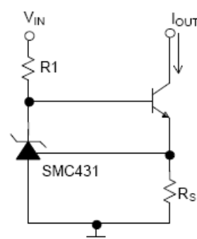
Fig. 21 Constant-Current Sink
