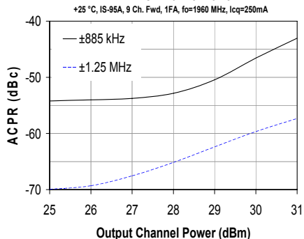
ACPR vs. Channel Power +25 °C, IS-95A, 9 Ch. Fwd, 1FA, fo=1960 MHz, I_{cq}=250 mA
