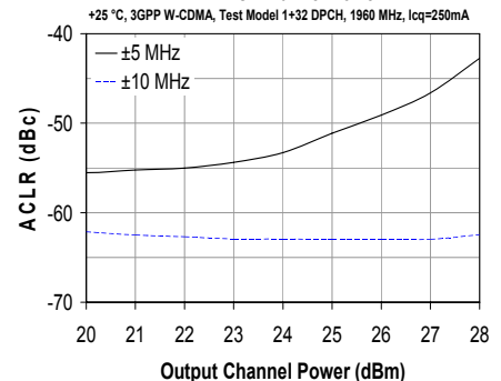
ACLR vs. Channel Power +25 °C, 3GPP W-CDMA, Test Model 1+32 DPCH, 1960 MHz, I_{cq}=250 mA
