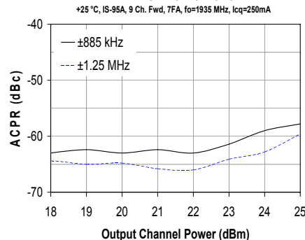
ACPR vs. Channel Power +25 °C, IS-95A, 9 Ch. Fwd, 7FA, fo=1935 MHz, I_{cq}=250 mA
