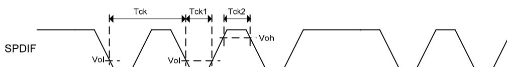
Figure 22. SPDIF Output Timing
