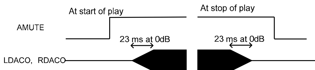
Figure 13. Waveform at Audio Mute
