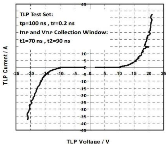
Figure 5 TLP V-I Curve
