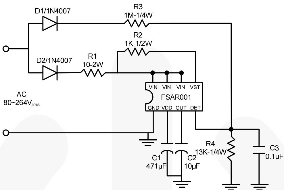
Figure 1. Typical Application
