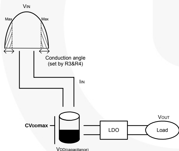
Figure 17. Operating Principle
