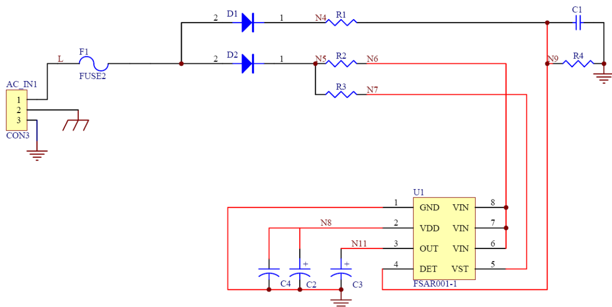
Figure 20. Application Circuit
