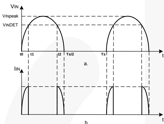
Figure 18. Typical Waveforms
