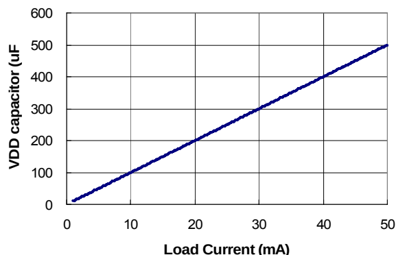
Figure 19. V_{DD} Capacitor vs. Output Current
