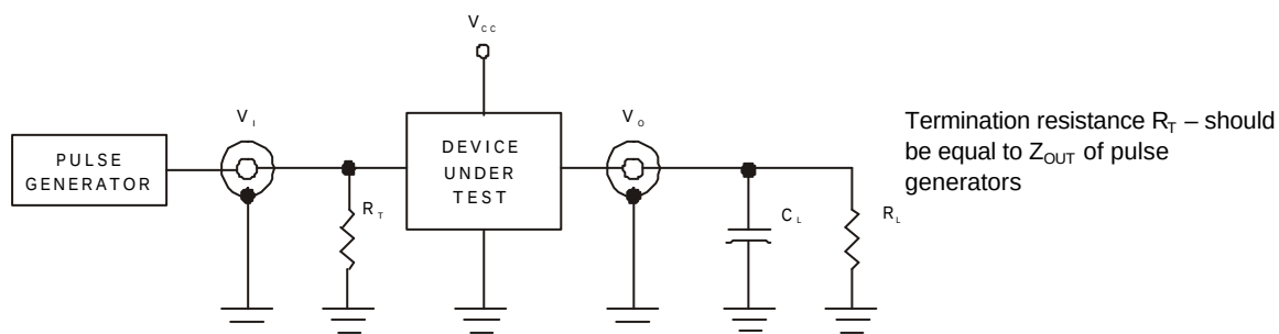
Figure 2. Test Circuit
