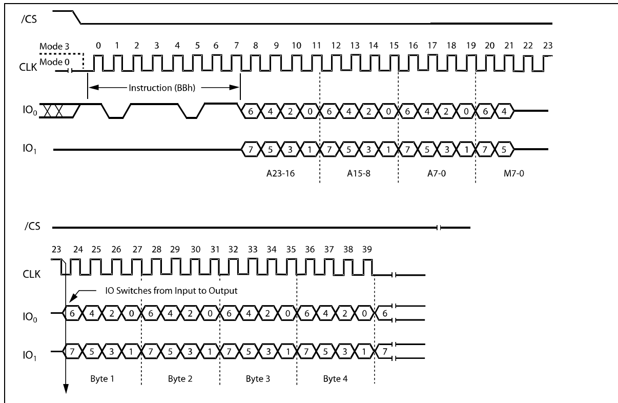
Figure 12a. Fast Read Dual I/O Instruction Sequence (Initial instruction or previous M5-4 \neq 10)
