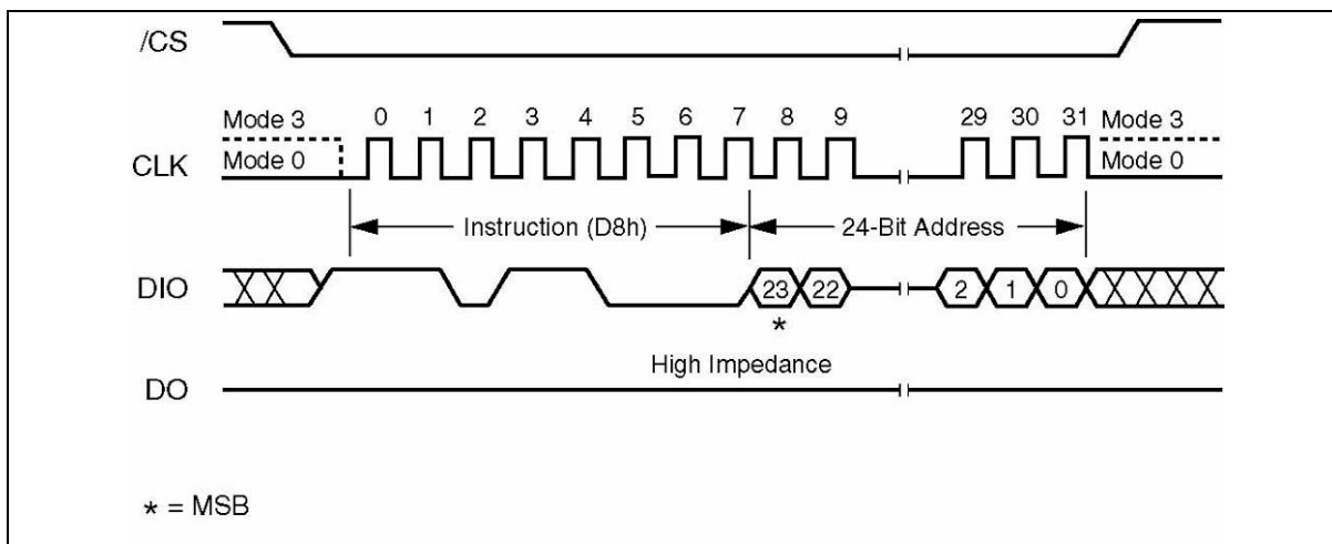
Figure 17. Block Erase Instruction Sequence Diagram
