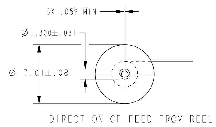
TAPE STYLE "SP" & "RP" 14
