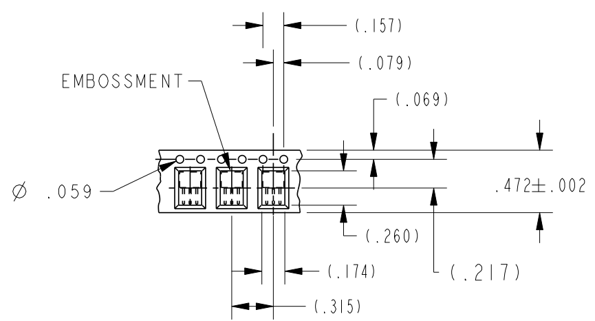
TAPE STYLE "SP" & "RP" 14
