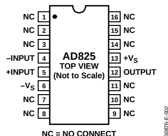
Figure 5. 16-Lead SOIC
