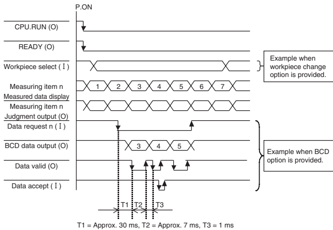
Timing Chart (Judgment output mode Y00)
