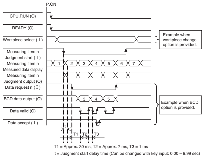
Timing Chart (Judgment output mode Y10)
