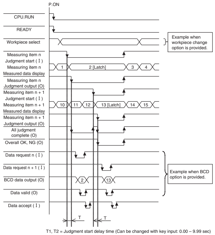
Timing Chart (Judgment output mode Y11)
