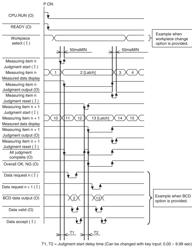
Timing Chart (Judgment output mode Y21)
