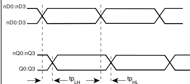
PROPAGATION DELAY
