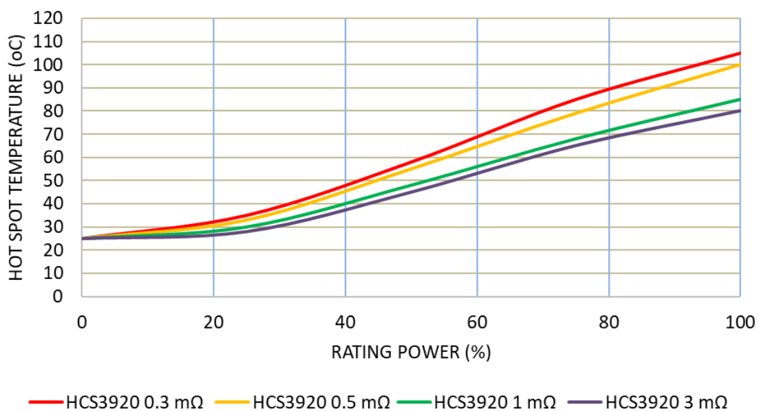
Rated Power vs. Surface Temperature – HCS3920
