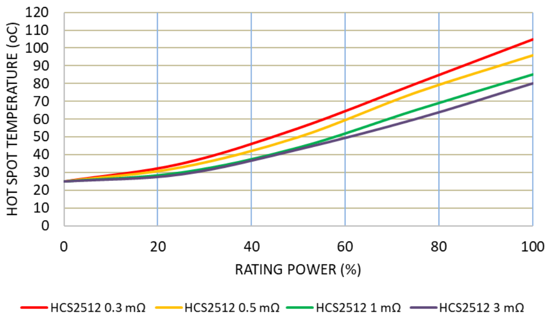
Rated Power vs. Surface Temperature – HCS2512
