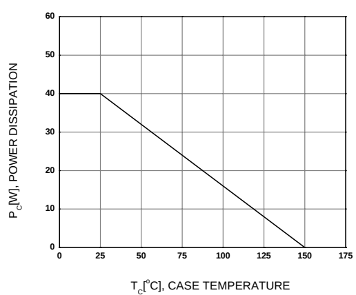
Figure 12. Power Derating
