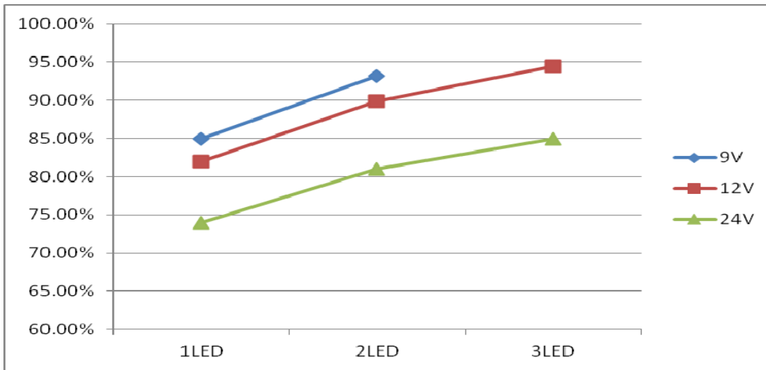
Efficiency vs. LED cascaded number @L=22uH, I_{OUT}=384\text{mA}
