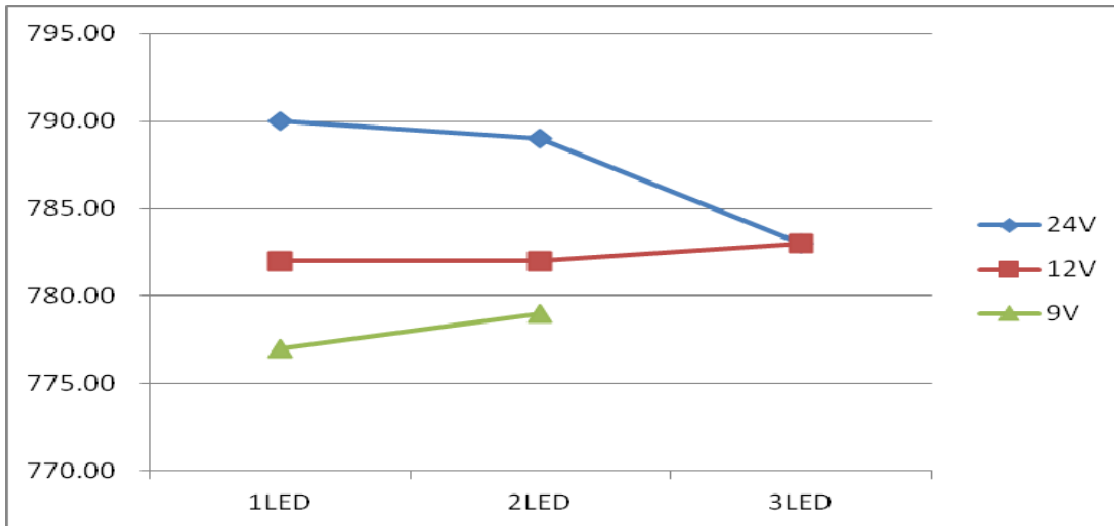
Output current vs. LED cascaded number @L=68uH, I_{OUT}=769\text{mA}
