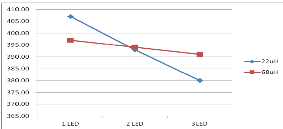
Output Current vs. LED Cascaded number @VIN=12V, I_{OUT}=384\text{mA}
