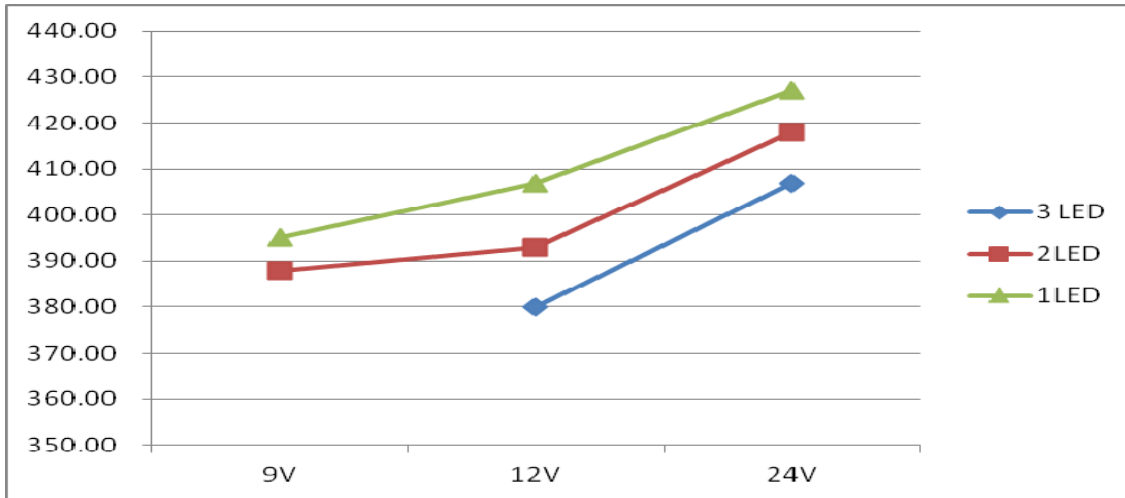
Output current vs. input voltage @L=22uH, I_{OUT}=384mA
