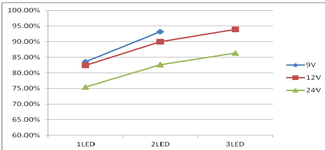
Efficiency vs. LED cascaded number @L=22uH, I_{OUT}=769\text{mA}
