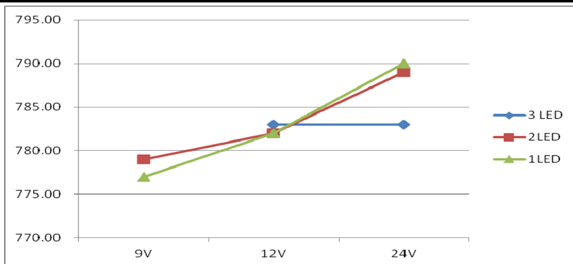
Output current vs. input voltage @L=68uH, I OUT =769mA
