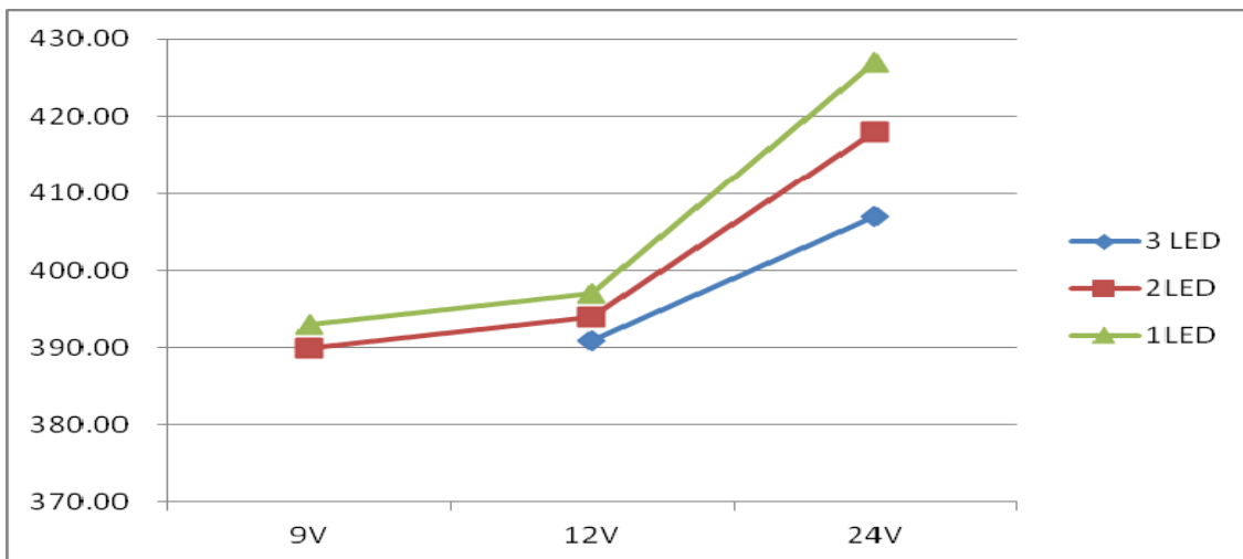
Output current vs. input voltage @L=68uH, I_{OUT}=384mA
