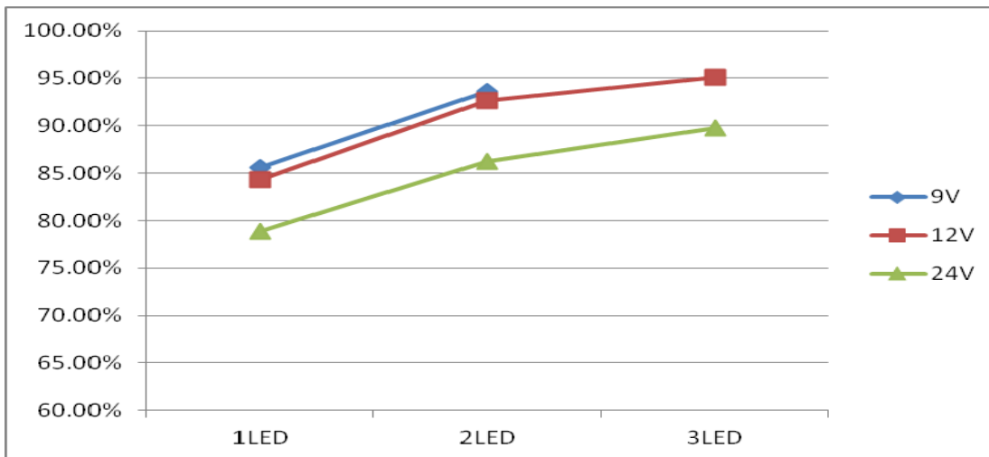
Efficiency vs. LED cascaded number @L=68uH, I_{OUT}=384\text{mA}
