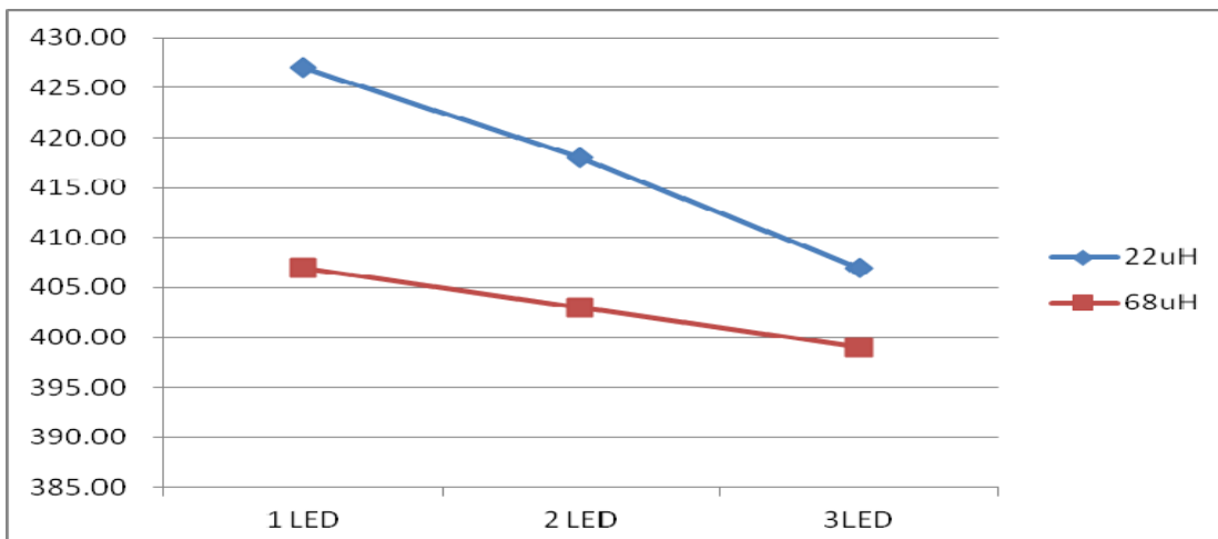
Output Current vs. LED Cascaded number @VIN=24V, I_{OUT}=384\text{mA}
