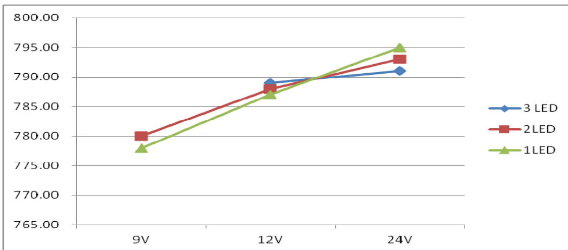
Output current vs. input voltage @L=22uH, I_{OUT}=769mA
