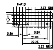
1 Form C (3.5 mm Pinning)
