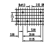
1 Form C (5 mm Pinning)
