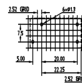
1 Form A (5 mm Pinning)
