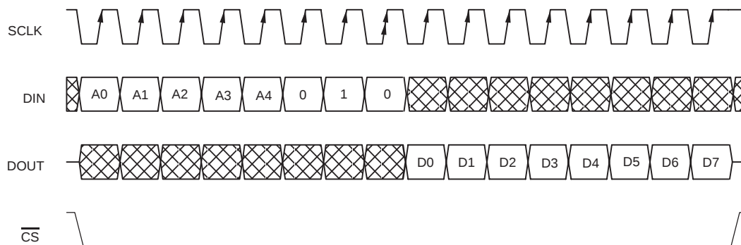
Figure 18. Timing Diagram for an 8-Bit Read Operation
