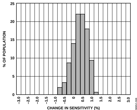
Figure 8. SOIC_CAV Sensitivity Error @ 25°C
