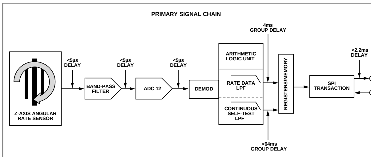
Figure 21. Primary Signal Chain and Associated Delays
