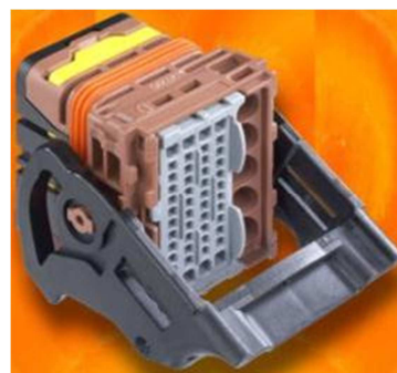
CMC Connectors 22, 28 and 53-circuits, 64326, 64318 and 64321 series
