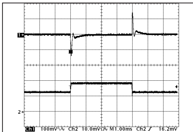
Figure 16: Output voltage response to step-change in load current (50%-75%-50% of Iout(max); dI/dt = 5A/μs). Load cap: 470μF, 30 mΩ ESR tantalum cap and 1μF ceramic cap. Ch 1: Vout (100mV/div), Ch 2: Iout (10A/div).
