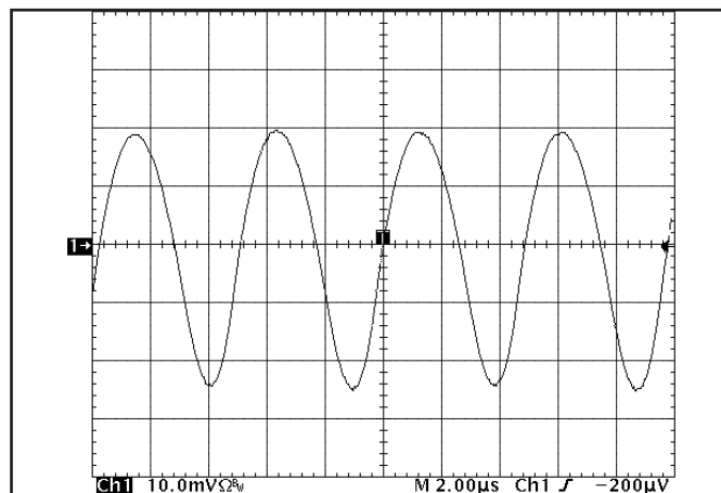
Figure 18: Input Terminal Ripple Current, i_c , at full rated output current and nominal input voltage with 10\ \mu\text{H} source impedance and 47\ \mu\text{F} electrolytic capacitor (200 mA/div). See Figure 17.
