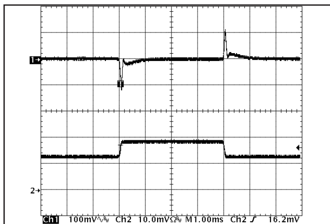
Figure 15: Output voltage response to step-change in load current (50%-75%-50% of Iout(max); dI/dt = 0.1A/μs). Load cap: 10μF, 100 mΩ ESR tantalum cap and 1μF ceramic cap. Ch 1: Vout (100mV/div), Ch 2: Iout (10A/div).
