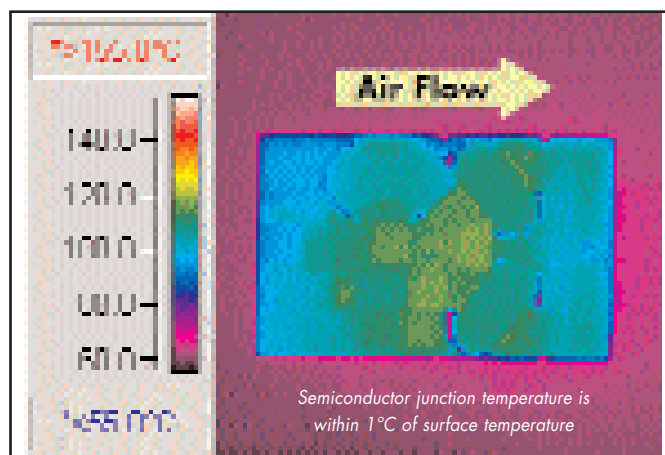
Figure 12: Thermal plot of converter at 25 amp load current with 55°C air flowing at the rate of 200 LFM. Air is flowing across the converter sideways from input to output (48V input).
