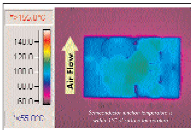
Figure 6: Thermal plot of converter at 25 amp load current with 55°C air flowing at the rate of 200 LFM. Air is flowing across the converter sideways from pin 3 to pin 1 (24V input).
