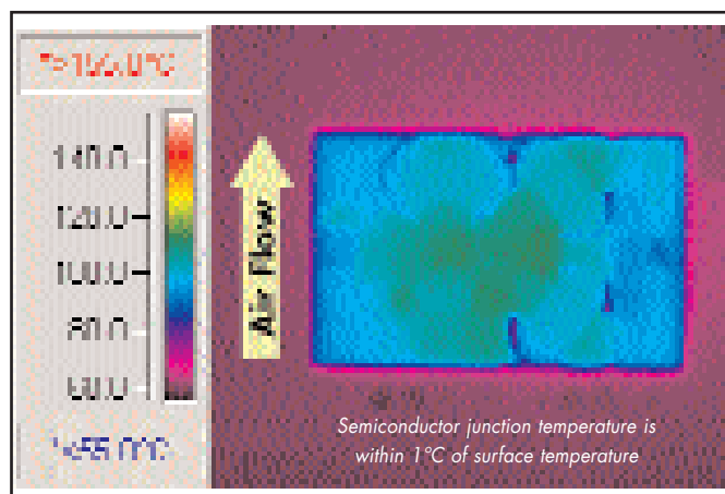
Figure 8: Thermal plot of converter at 25 amp load current with 55°C air flowing at the rate of 200 LFM. Air is flowing across the converter sideways from pin 3 to pin 1 (48V input).
