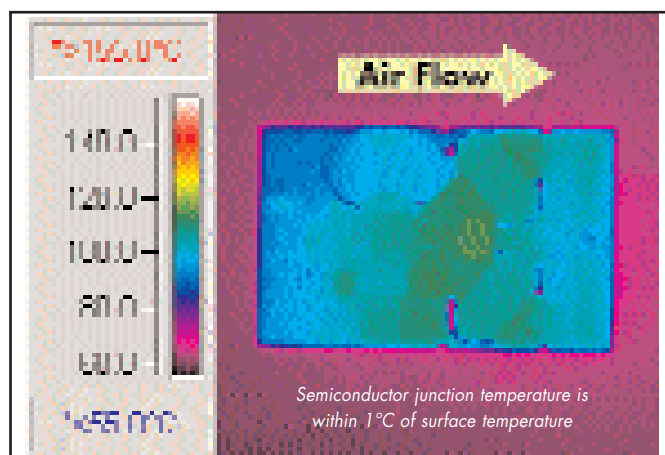
Figure 10: Thermal plot of converter at 25 amp load current with 55°C air flowing at the rate of 200 LFM. Air is flowing across the converter sideways from input to output (24V input).
