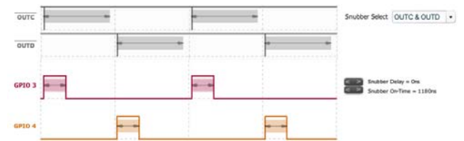
Figure 46. Active Clamp Snubber Configured on OUTx Signals
