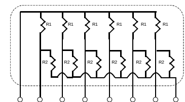
Fig. 6: TERMINATION CIRCUIT
