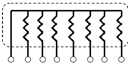
Fig. 1: BUSSED/COMMON CIRCUIT
