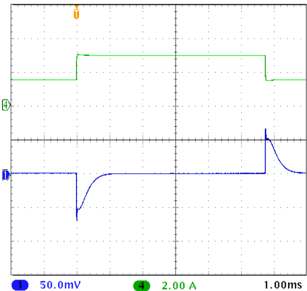
UNITS ARE PER DIVISION, 10 µs SLEW RATE MWR28515T STEP LOAD MAIN, 50% - 100% - 50% FIGURE 7
