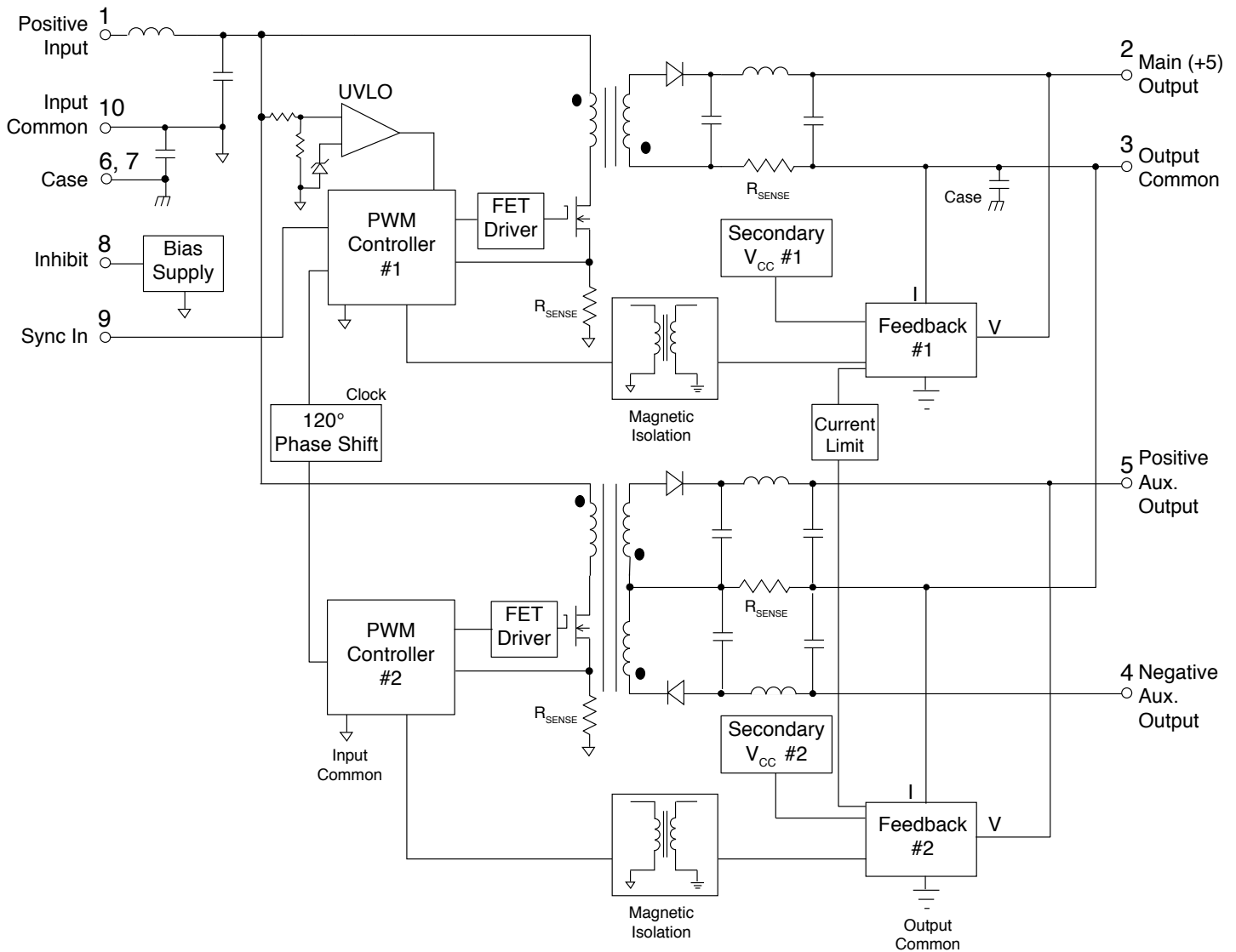
FIGURE 1: MWR BLOCK DIAGRAM
