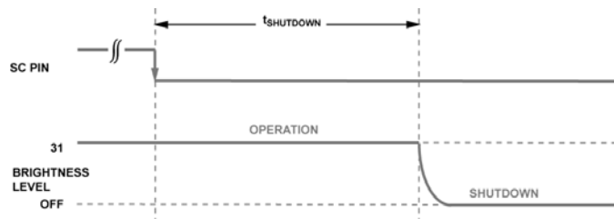
Figure 4. Shutdown Timing
