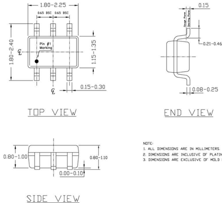
6-Pin SC-70 (C6)
