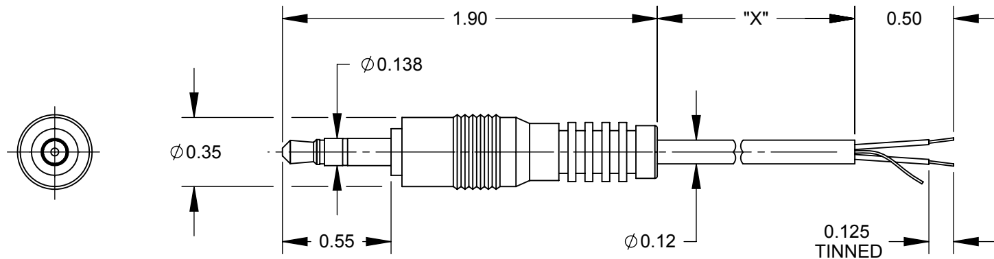
3.5MM STEREO PLUG
