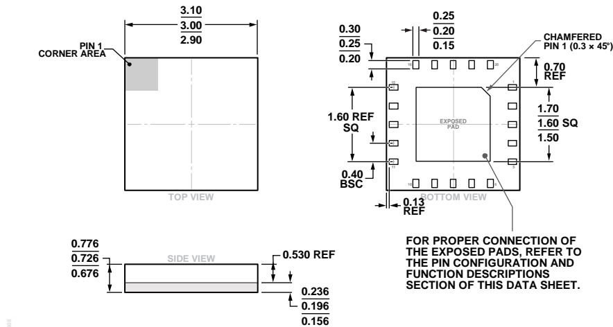
Figure 24. 20-Terminal Land Grid Array [LGA] 3 mm x 3 mm Body and 0.72 mm Package Height (CC-20-3) Dimensions shown in millimeters
