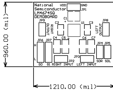
Figure 37. Top Silkscreen
