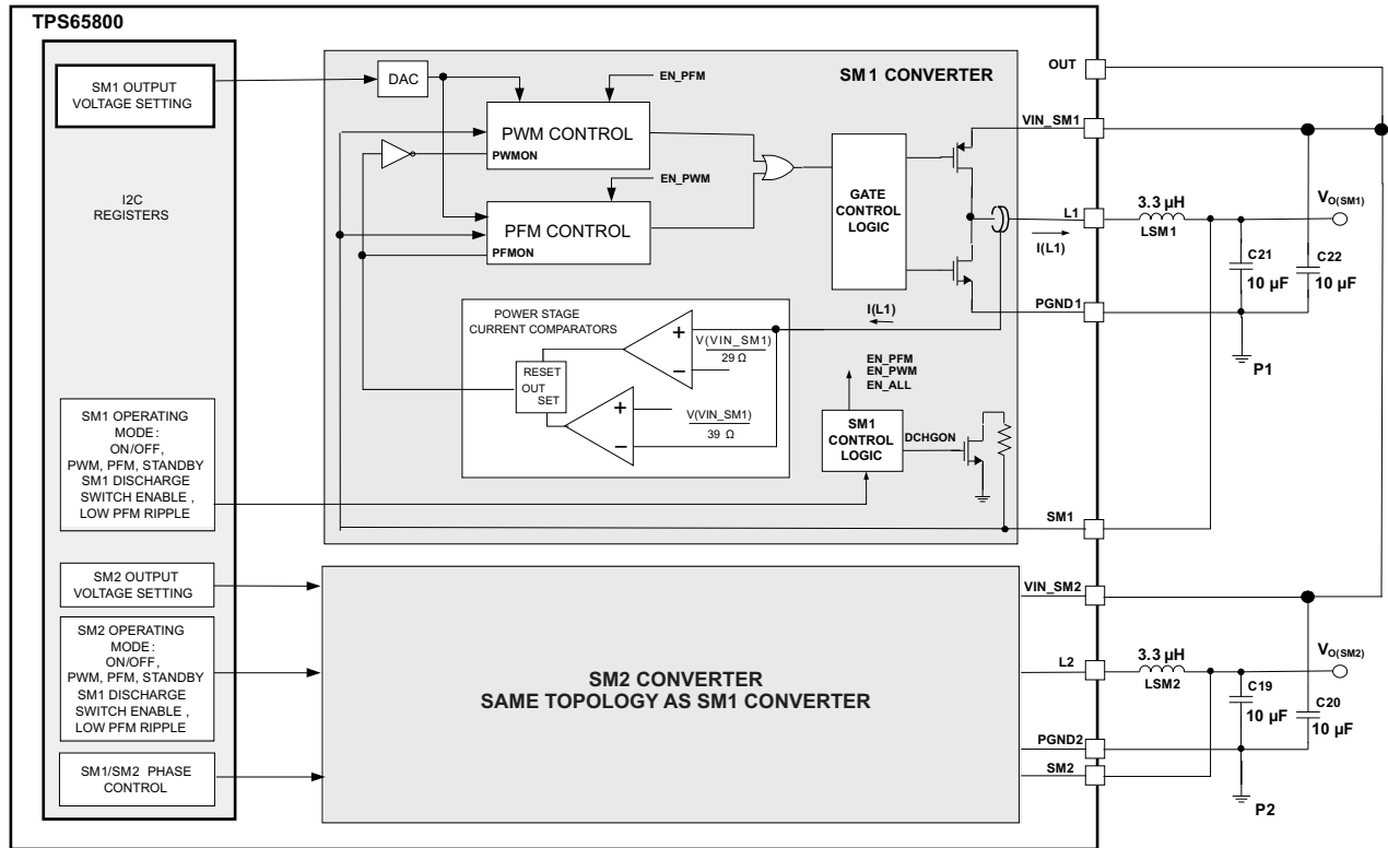
Figure 41. SM1/SM2 Converter
