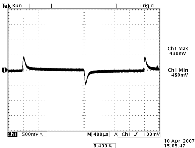
Photo 11: Transient Response – 0.1A/us Vin=24 V, Iout = 1 to 3 A (25% to 75%) With a 22 uF Tantalum across the Output
