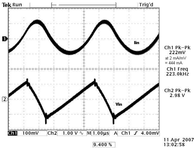
Photo 1: Input Ripple Voltage and Current Vin=24 V, Iout = 4 A
