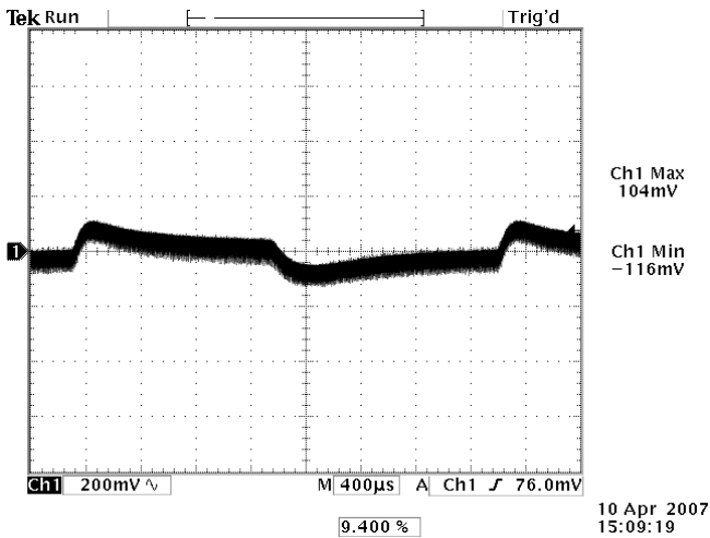
Photo 9: Transient Response – 0.01 A/us Vin=24 V, Iout = 1 to 3 A (25% to 75%)
