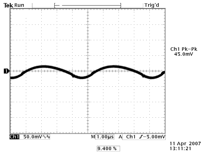
Photo 8: Output Ripple and Noise (20 MHz BW) Vin=24 V, Iout = 2.5 A With a 22 uF Tantalum across the Output
