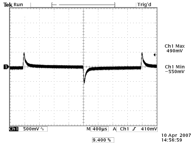
Photo 10: Transient Response – 0.1 A/us Vin=24 V, Iout = 1 to 3 A (25% to 75%)
