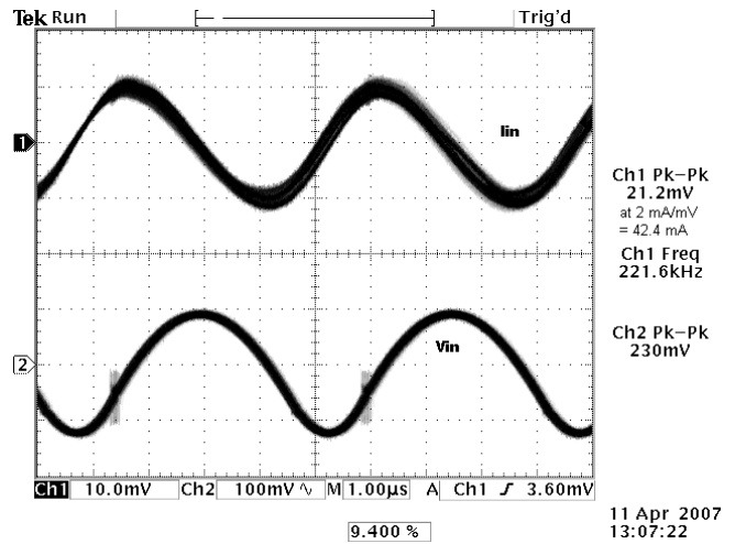
Photo 2: Input Ripple Voltage and Current Vin=24 V, Iout = 4 A With a 120 µF Aluminum Electrolytic across the Input
