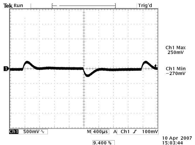
Photo 12: Transient Response – 0.1A/us Vin=24 V, Iout = 1 to 3 A (25% to 75%) With a 470 uF Electrolytic across the Output
