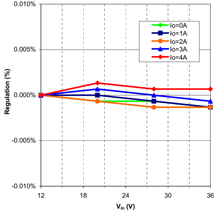
Graph 8: MPQ24S15-50C Line Regulation (+SENSE to +Vout, -SENSE to -Vout)
