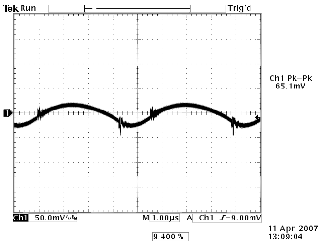
Photo 7: Output Ripple and Noise (20 MHz BW) Vin=24 V, Iout = 2.5 A
