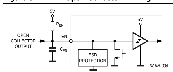
Figure 8. EN Pin Open Collector Driving
