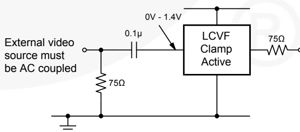
Figure 17. SCART with DC-Coupled Outputs
