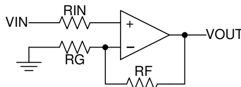
Figure 45. Operational Amplifier Schematic for Noninverting Configuration
