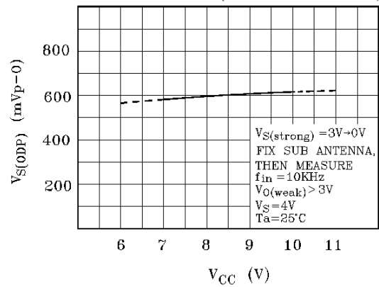
ODP SENSITIVITY - V_{CC} (CONTINUOUS WAVE)
