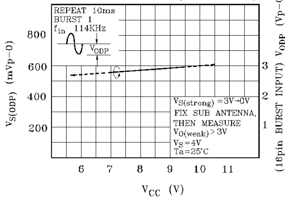
ODP SENSITIVITY - V_{CC} (TONE BURST)
