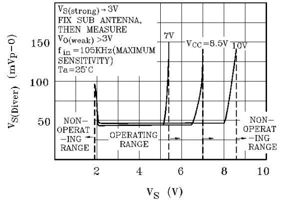
DIVERSITY INPUT SENSITIVITY - V_S (CONTINUOUS WAVE)
