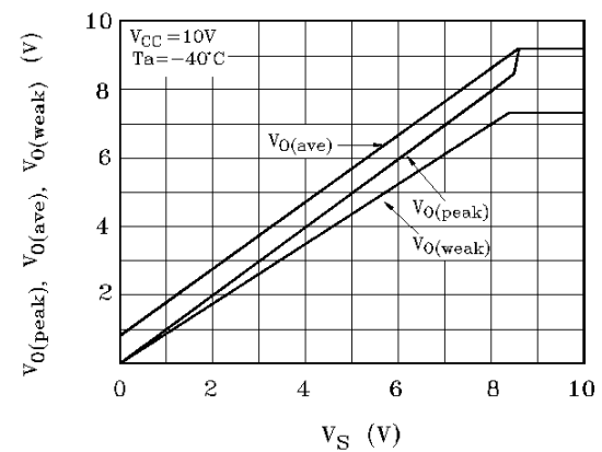
V_O(\text{peak}) , V_O(\text{ave}) , V_O(\text{weak}) - V_S
