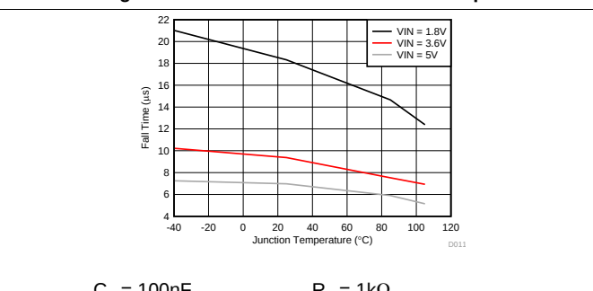
Figure 10. Fall Time vs Junction Temperature
