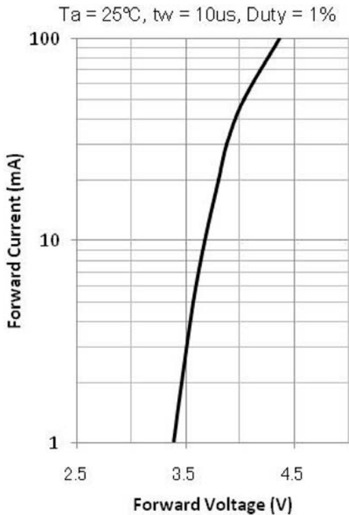
Forward Current – Forward Voltage
