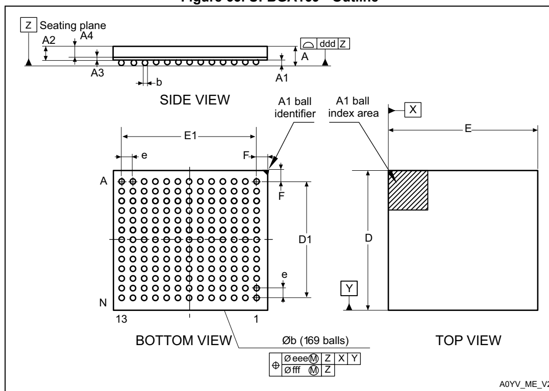
Figure 63. UFBGA169 - Outline
