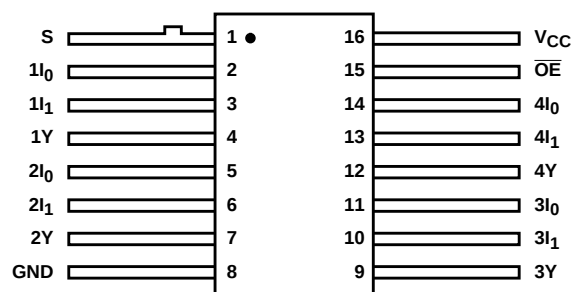
ACS257 (FLATPACK) TOP VIEW
