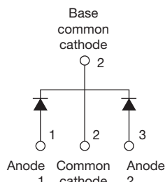
VS-MURB1020CT-1PbF
