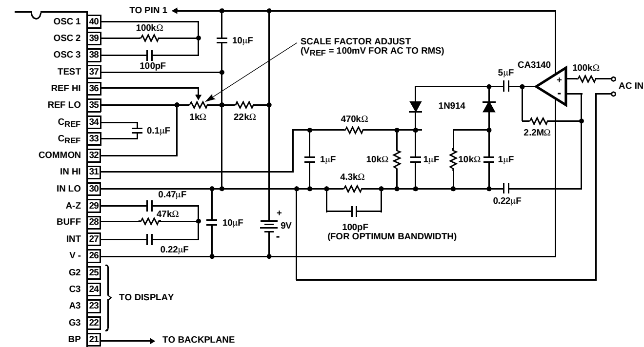
FIGURE 12. AC TO DC CONVERTER WITH HI7106
