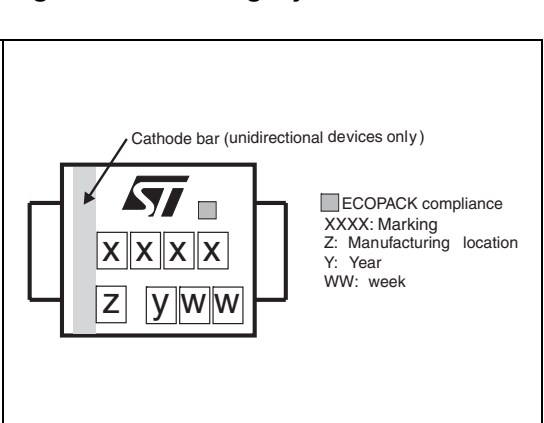
Figure 18. Marking layout (1)
