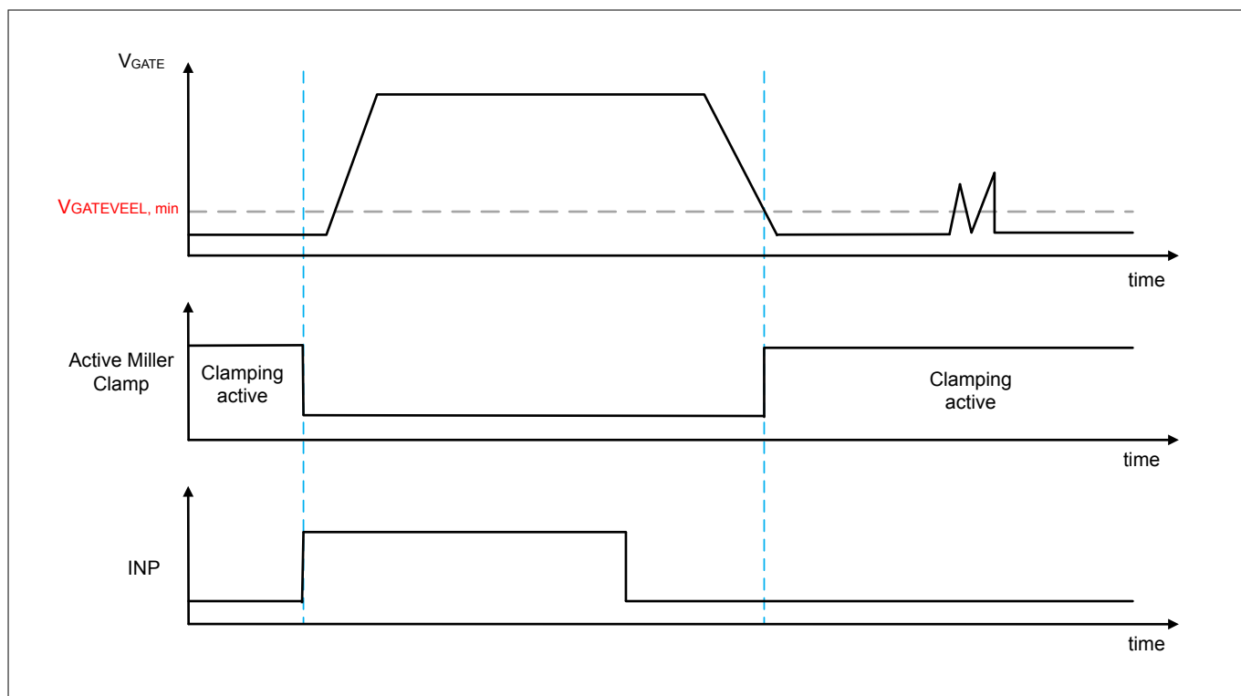
Figure 16 Active Miller clamp timing diagram
