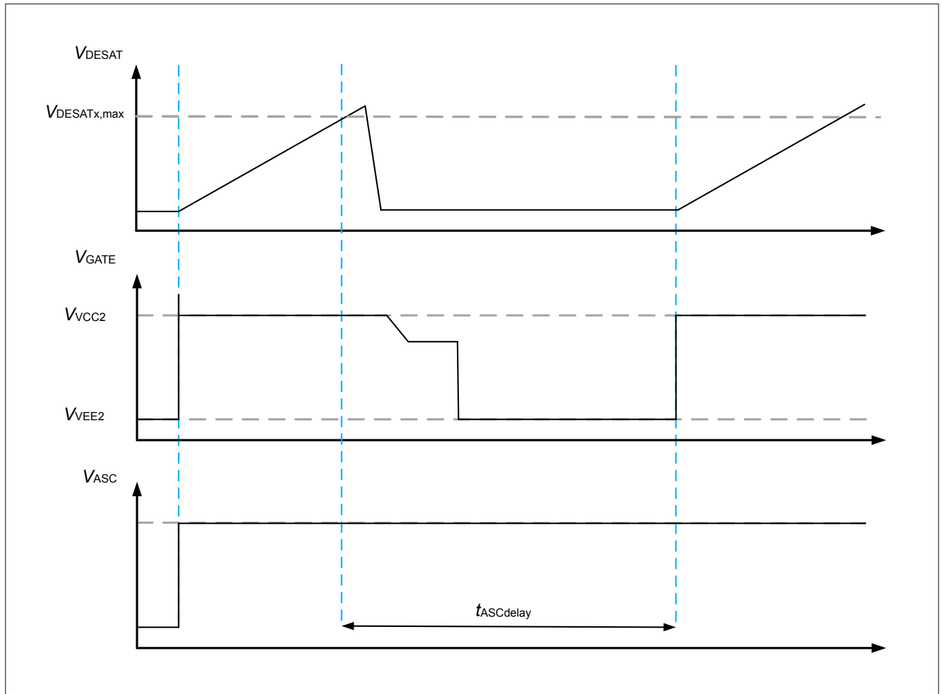
Figure 17 ASC turn-on delay after ASC trigger with DESAT/OC event
