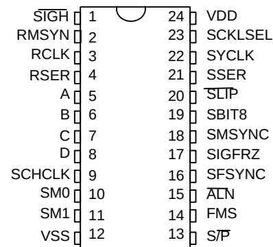
24-PIN 300 MIL DIP
