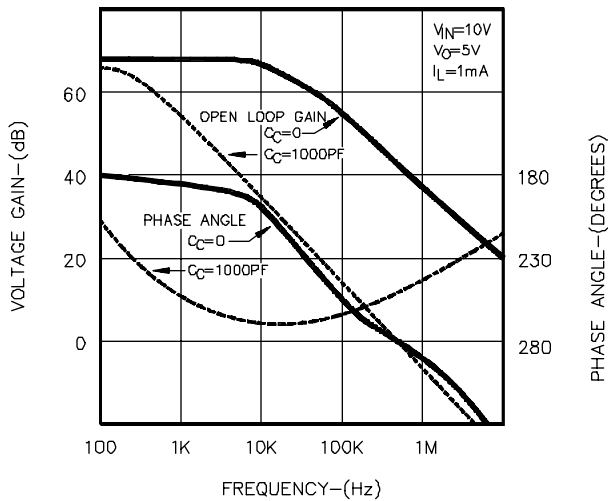
FIGURE 5. FREQUENCY RESPONSE
