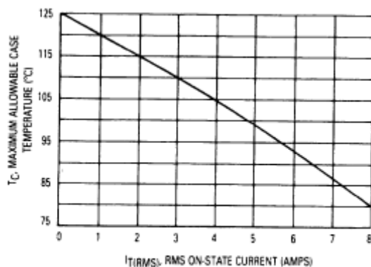
Figure 1. Current Derating
