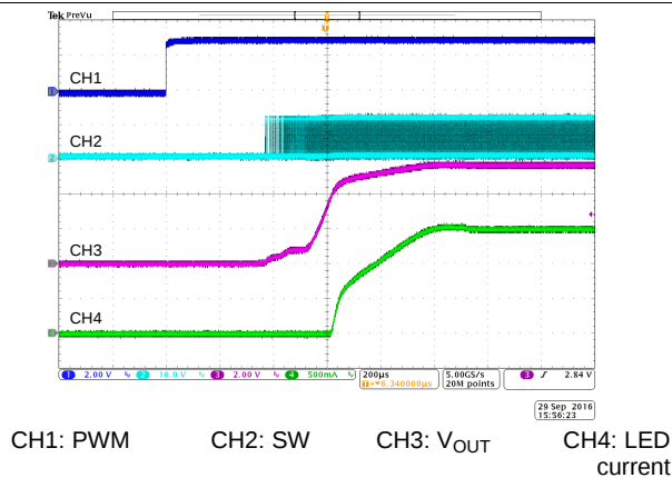
图 30. Start-Up at 1% PWM Duty Cycle and 50 kHz
