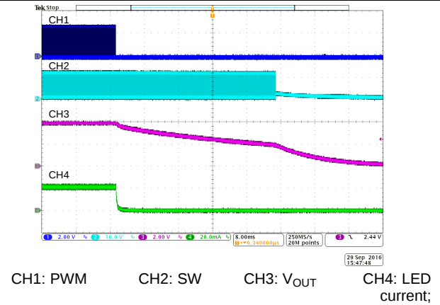
图 31. Shutdown at 1% PWM Duty Cycle and 50 kHz
