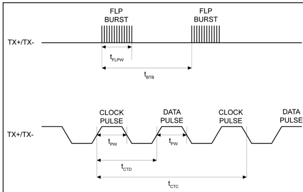
Figure 23: Auto-Negotiation Timing
