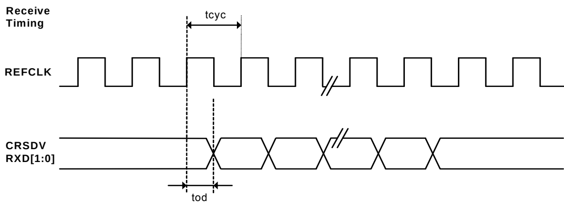
Figure 20. RMII Timing – Data Transmitted to RMII
