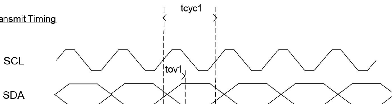
Figure 14. EEPROM Interface Output Transmit Timing Diagram
