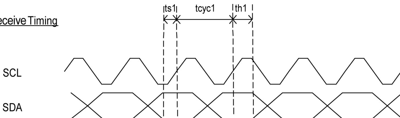
Figure 13. EEPROM Interface Input Receive Timing Diagram
