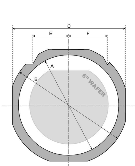
Figure 12 FF070 Frame with a 6 inch wafer
