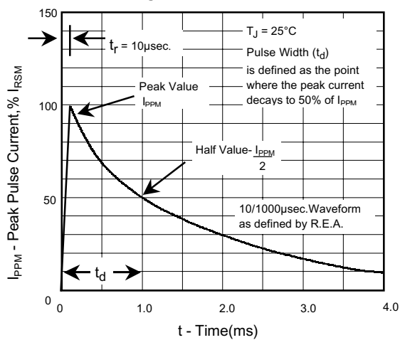
Fig.3 - Pulse Waveform
