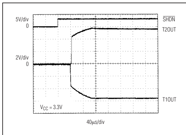
Figure 7. MAX3111E Transmitter Outputs Exiting Shutdown or Powering Up
