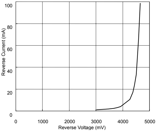
ZD5229A Reverse Current vs Reverse Voltage
