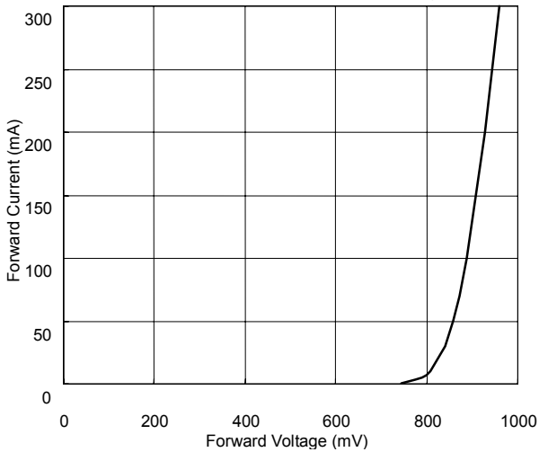
ZD5229A Forward Current vs Forward Voltage
